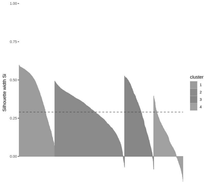
Silhouette Plot - K-Means Clustering
